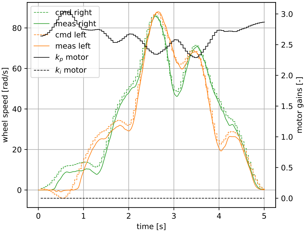
Wheel Speeds
